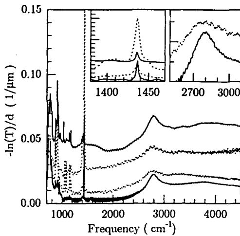
Figure 1: Solid lines: \text{YBa}_2\text{Cu}_3\text{O}_{6+x} (with x \approx 0 and x \ll 0.1 ); dotted lines: \text{YBa}_2(\text{Cu}_{0.95}\text{Zn}_{0.05})_3\text{O}_6 ; T=4\text{K} .
