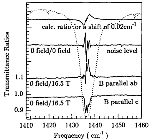
Figure 2: Dotted line: Transmittance of the sharp peak at 1436\text{ cm}^{-1} for T=1\text{K} . Solid lines: Calculated (topmost) and measured ratios of transmission data for different values of the external magnetic field.
